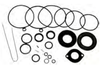
18-8361 UPPER SEAL KIT Replaces: 576266-8 For: AQ200-AQ290
