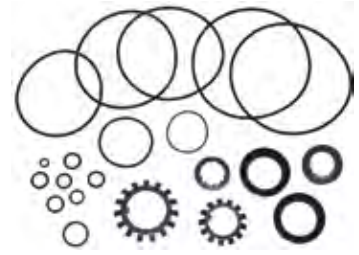
18-8359 LOWER GEARCASE SEAL KIT Replaces: 876268 For: AQ200-AQ290
