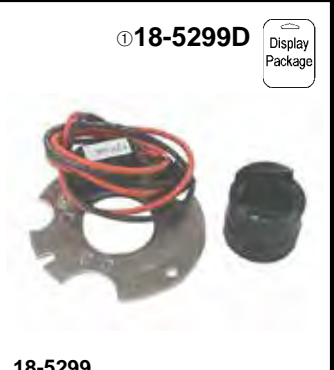
18-5299D ELECTRONIC CONVERSION KIT Fits: 8 (Cyl.) AQ200A, B, AQ225A, B and All 8 Cyl. w/Prestolite Dist # IBM-7013A Use with 18-5403 style rotor
