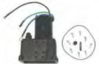
18-6763 TILT/TRIM MOTOR Replaces: 92975A6, 79271A4, 67914A2, 92975A32, 93247A7 To 1984. Fits most Mercruiser Sterndrives (Motor and Reservoir Only) For Repair Kit use: 18-6253
