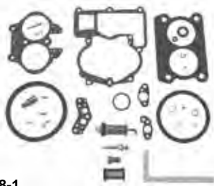
18-7098-1 CARB KIT Replaces 3302-804844002 MerCarb 2 bbl. side fill accelerator pump 1986 and UP MCM 4-cyl., V6 & V8
