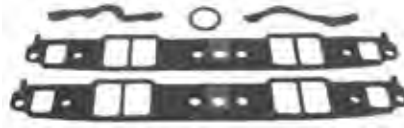
18-0868 INTAKE MANIFOLD GASKET SET Replaces: 27-17145 For: Mercruiser 305, 350
