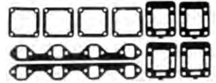
18-4399 EXHAUST MANIFOLD GASKET SET Replaces: 27-54566A1 For: Ford 302/351 (5.0L & 5.8L) CID Eng; All 888 (188 HP) & 233 HP, 255 HP S/N 3258728-4175498 — CONTAINS —
